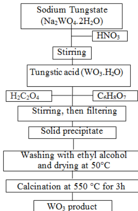
Figure 1: Schematic diagrams of steps involved in obtaining \text{WO}_3 powders
