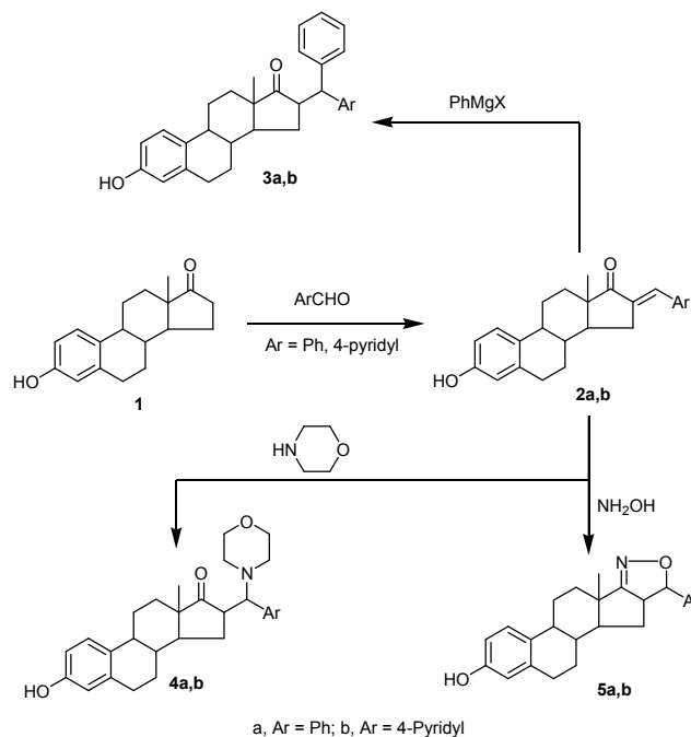
Scheme 1. Synthetic routes to starting compounds 2-5.
