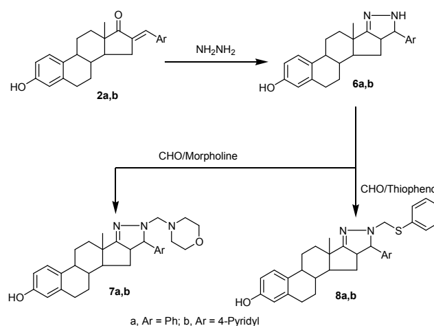
Scheme 2. Synthetic routes to starting compounds 6-8.
