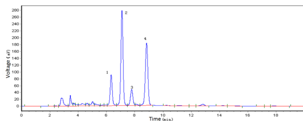
Figure 1. High-performance liquid chromatography plot of flavonoids from unprocessed Fructus aurantii .
