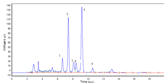
Figure 2. High-performance liquid chromatography plot of Fructus aurantii flavonoids after Zhangband processing: 2, naringin; 3, hesperindin; 4, neohesperindin; 6, hesperetin 7-O-β-D-glucopyranoside.
