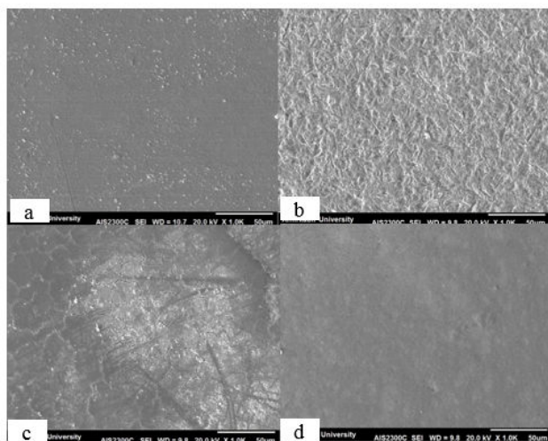
Figure 3. SEM micrographs of the surface of samples at ×1000 magnification: (a) control; (b) sandblasted group; (c) 9 J/cm² laser; (d) 5 J/cm² laser.
