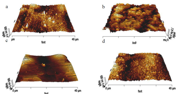
Figure 2. AFM micrographs (a) control; (b) sandblasted group; (c) 9 J/cm² laser; (d) 5 J/cm² laser.
