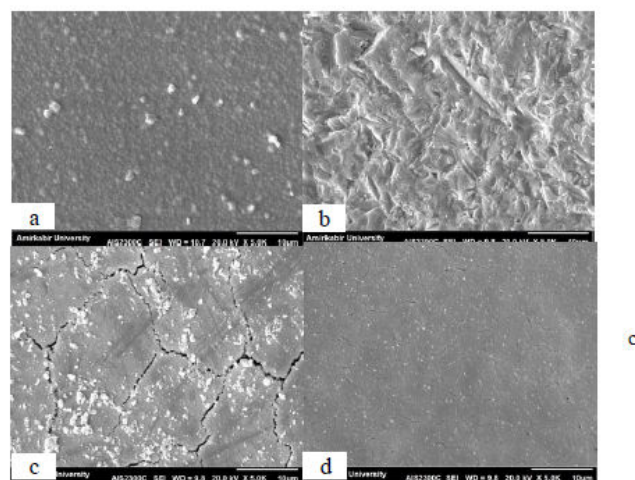
Figure 4. SEM micrographs of the surface of samples at x5000 magnification: (a) control; (b) sandblasted group; (c) 9 J/cm² laser; (d) 5 J/cm² laser.
