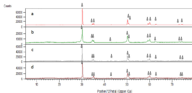
Figure 5. XRD diagram: (a) control; (b) sandblasted group; (c) 9 J/cm² laser; (d) 5 J/cm² laser.
