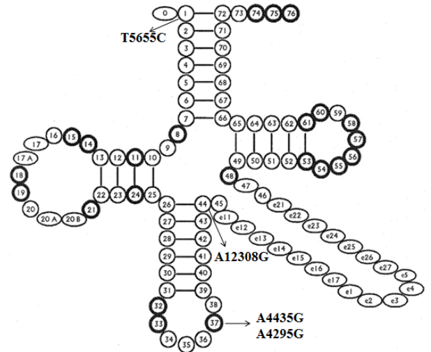
Figure 1. Cloverleaf structure of mt-tRNA with standard nucleotide numbering. The nucleotides in the variable stem have the prefix ‘e’ and are located between positions 45 and 46, obeying the base-pairing rules. Arrows indicate the position of T5655C, A4435G, A4295G and A12308G variants.
