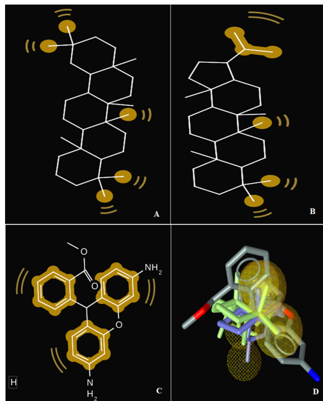
Figure 2. Structure of ligand (a) Zinc64624173, (b) Zinc64624174 (c) Zinc04099018 and (d) 3D structure of the pharmacophore molecule created with help of best three ligands.
